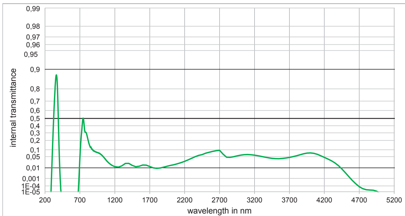
Internal transmittance \tau_i at reference thickness
